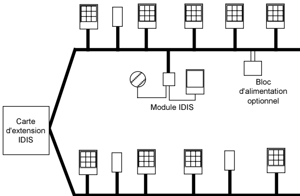
Figure 26. Configuration en "anneau"
