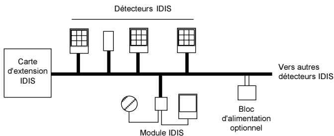
Figure 24. Configuration bus
